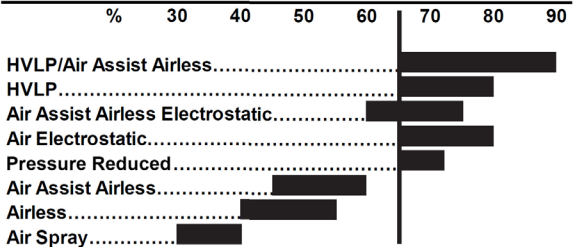
Baseline Transfer Efficiency of Coating Methods
